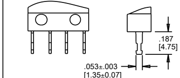
TERMINAL STYLE 3 TURRET, 3/16" LONG
