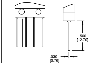
TERMINAL STYLE 4 WIRE WRAP
