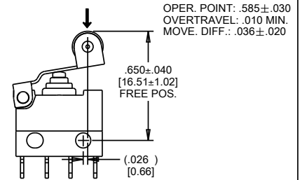
IN-LINE ROLLER LEVER (LEVER TYPE OPTION 3)
