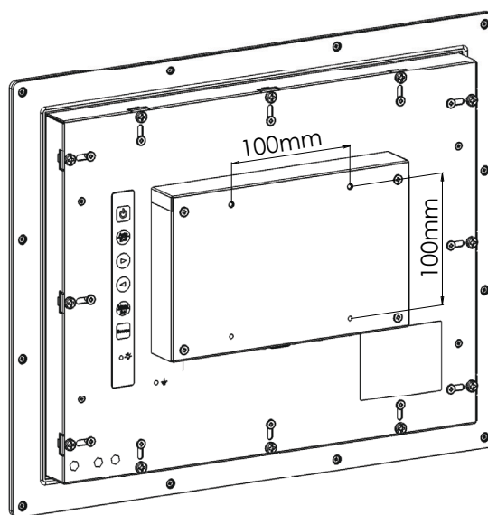
Figure 2.4 VESA Mounting
