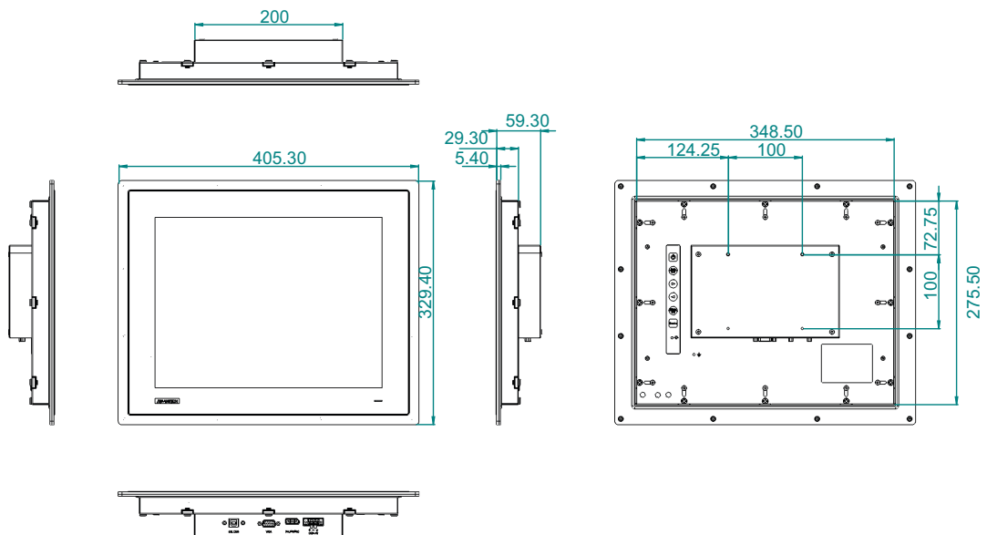
Figure 1.2 FPM-815S Dimensions
