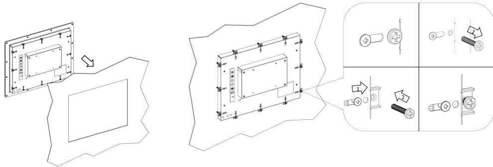
Figure 2.1 Panel Mounting
