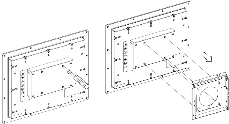
Figure 2.2 Wall Mounting
