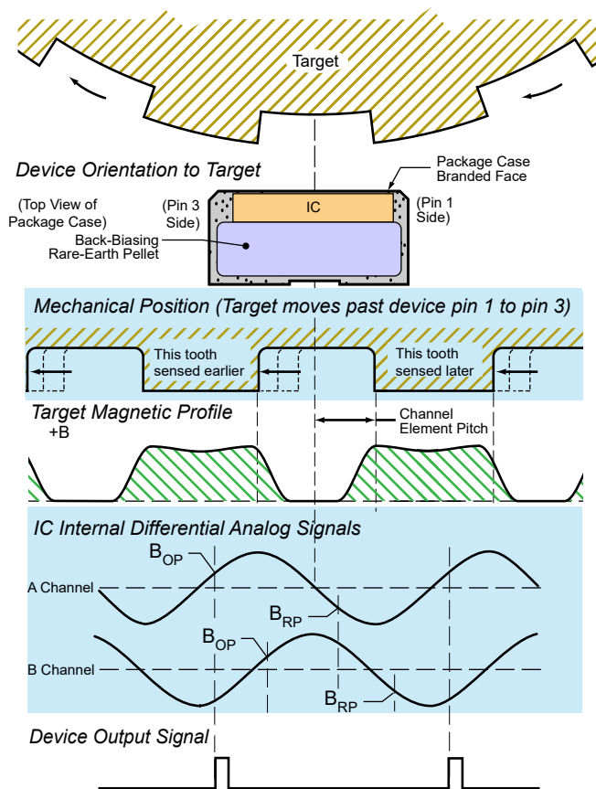
Figure 3: Magnetic Profile
