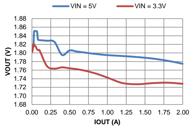
Figure 12. Load Regulation
