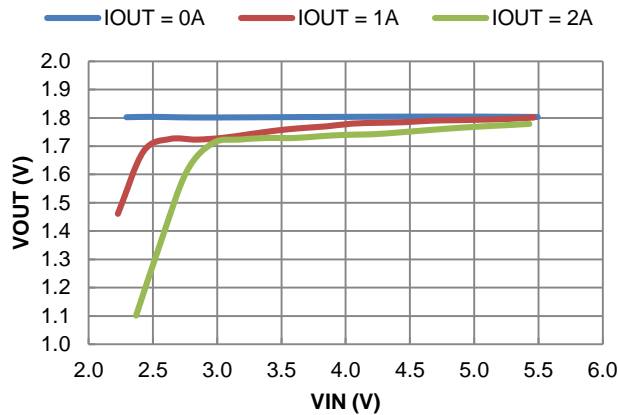
Figure 11. Line Regulation
