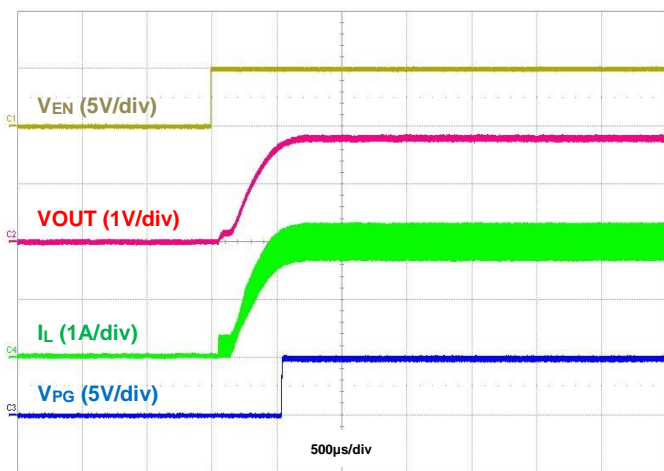
Figure 24. Startup Using EN, I_{OUT} = 2\text{A}
