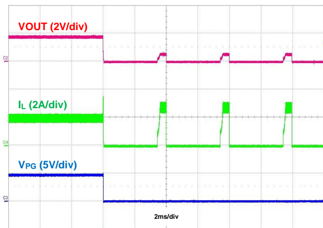
Figure 26. Output Short Protection, I_{OUT} = 2\text{A}
