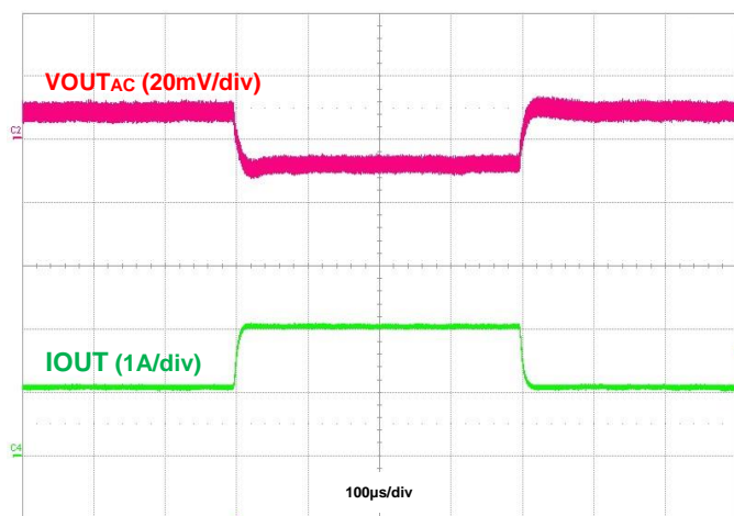
Figure 18. Load Transient, I_{OUT} = 1\text{A} to 2\text{A} to 1\text{A}
