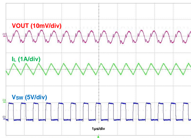
Figure 16. Output Voltage Ripple, I_{OUT} = 2\text{A}
