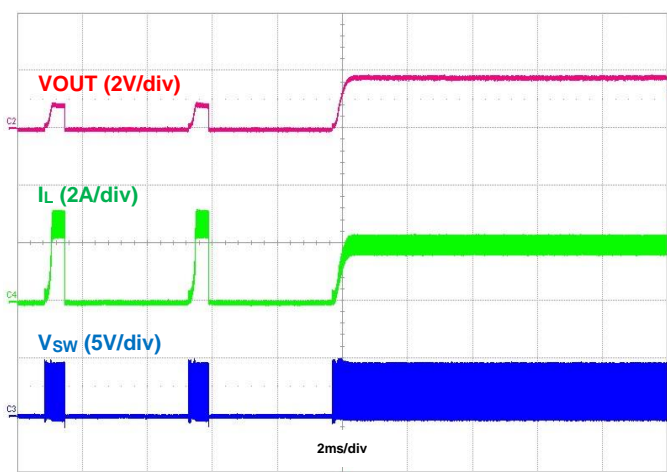
Figure 23. Output Short Recovery, IOU = 2A
