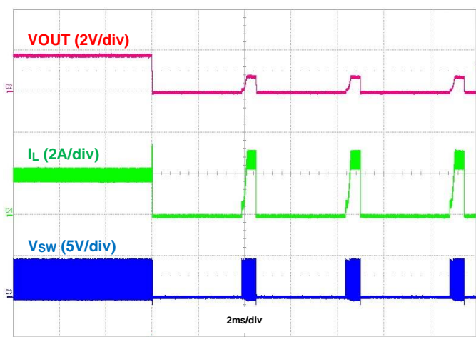
Figure 22. Output Short Protection, IOU = 2A
