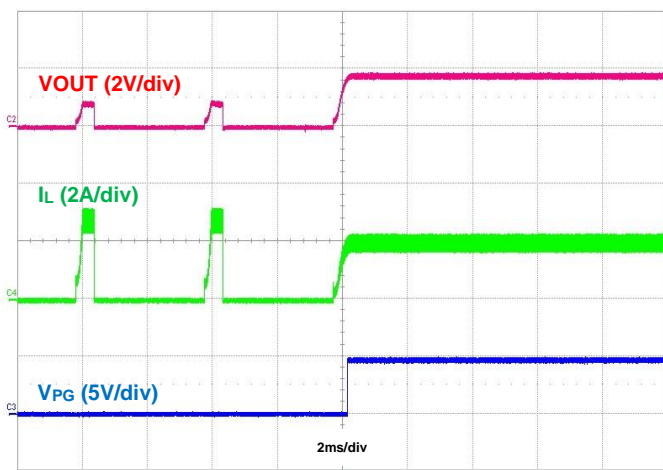
Figure 27. Output Short Recovery, I_{OUT} = 2\text{A}
