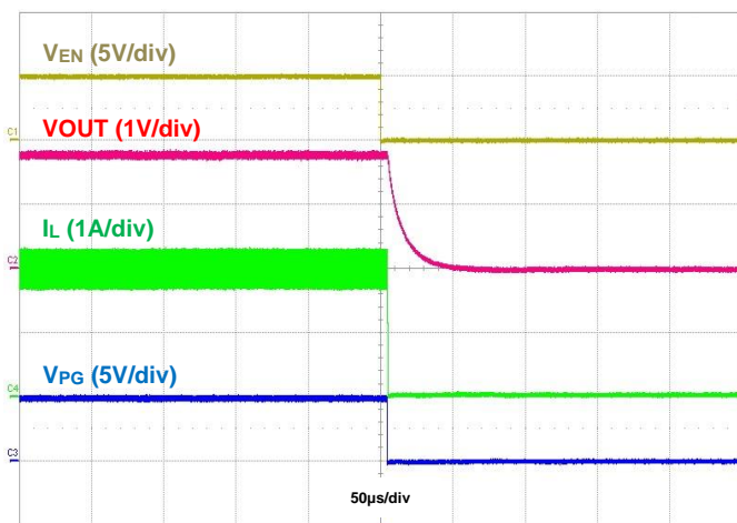
Figure 25. Shutdown Using EN, I_{OUT} = 2\text{A}
