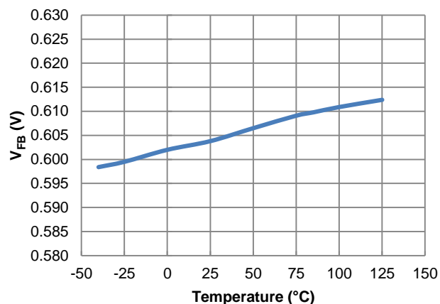
Figure 6. V_{FB} vs. Temperature
