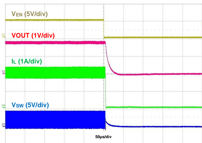
Figure 21. Shutdown Using EN, IOU = 2A
