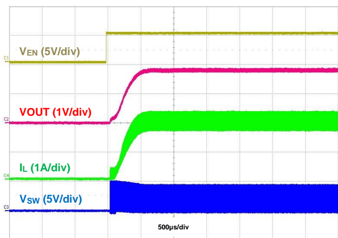
Figure 20. Startup Using EN, IOU = 2A
