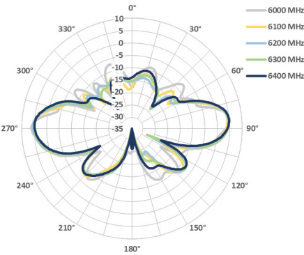
Phi 0° Plane
