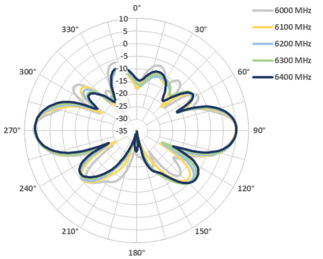
Phi 90° Plane
