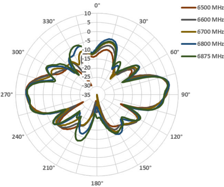
Phi 0° Plane
