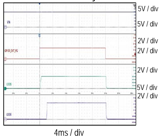
CMI 102 Enable LDO5/6 by GPIO7
