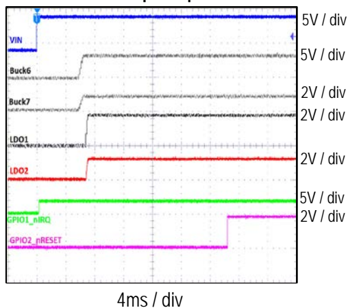
CMI 102 Startup Sequence
