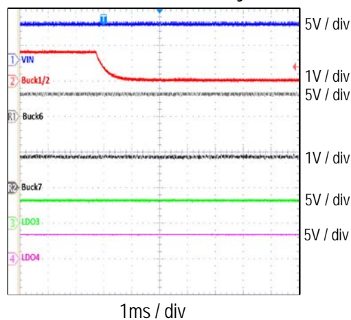
CMI 102 Enter SLEEP Mode by I2C
