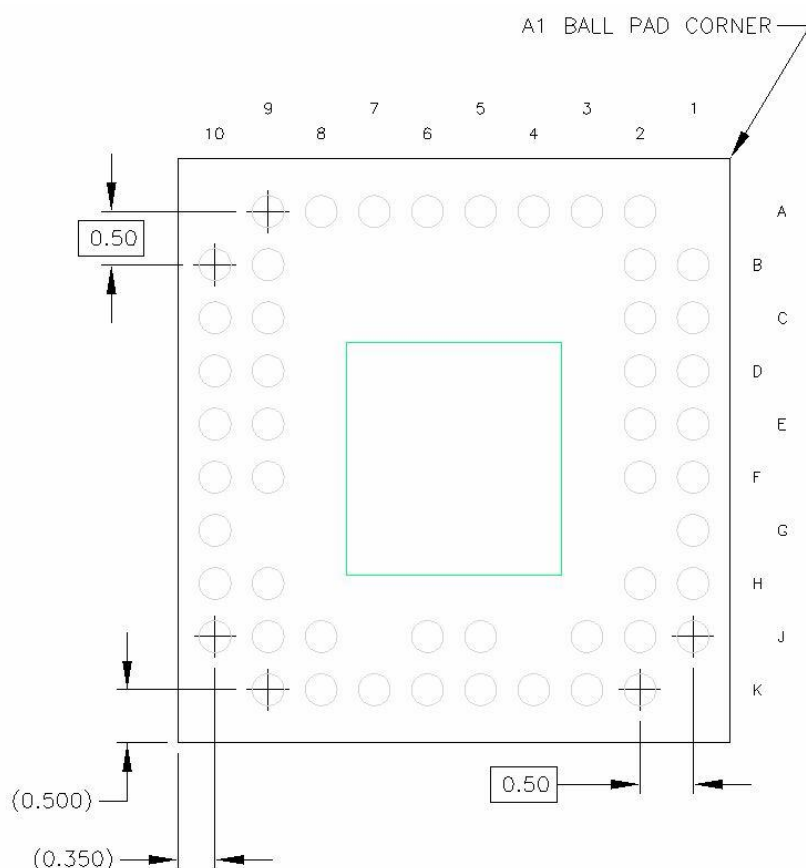
Figure 9.4. Physical layout of the A121 sensor, bottom view.
