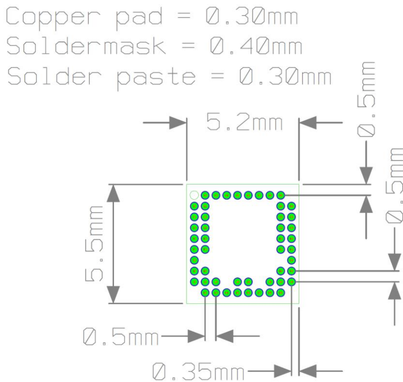
Figure 9.1. A121 footprint.
