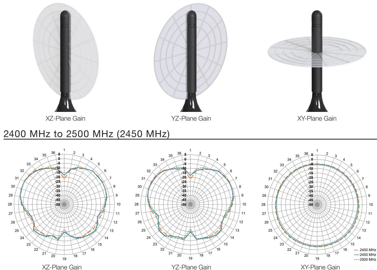
Figure 16. Radiation Patterns for ANT-2.4-MMG1-SMA Antenna, Free Space
