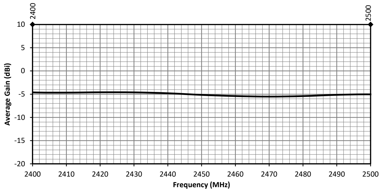
Figure 7. ANT-2.4-MMG1-SMA Antenna Average Gain on Ground Plane
