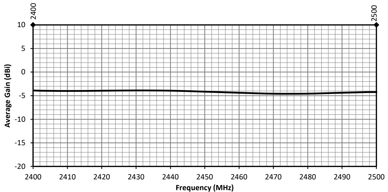
Figure 14. ANT-2.4-MMG1-SMA Antenna Average Gain, Free Space
